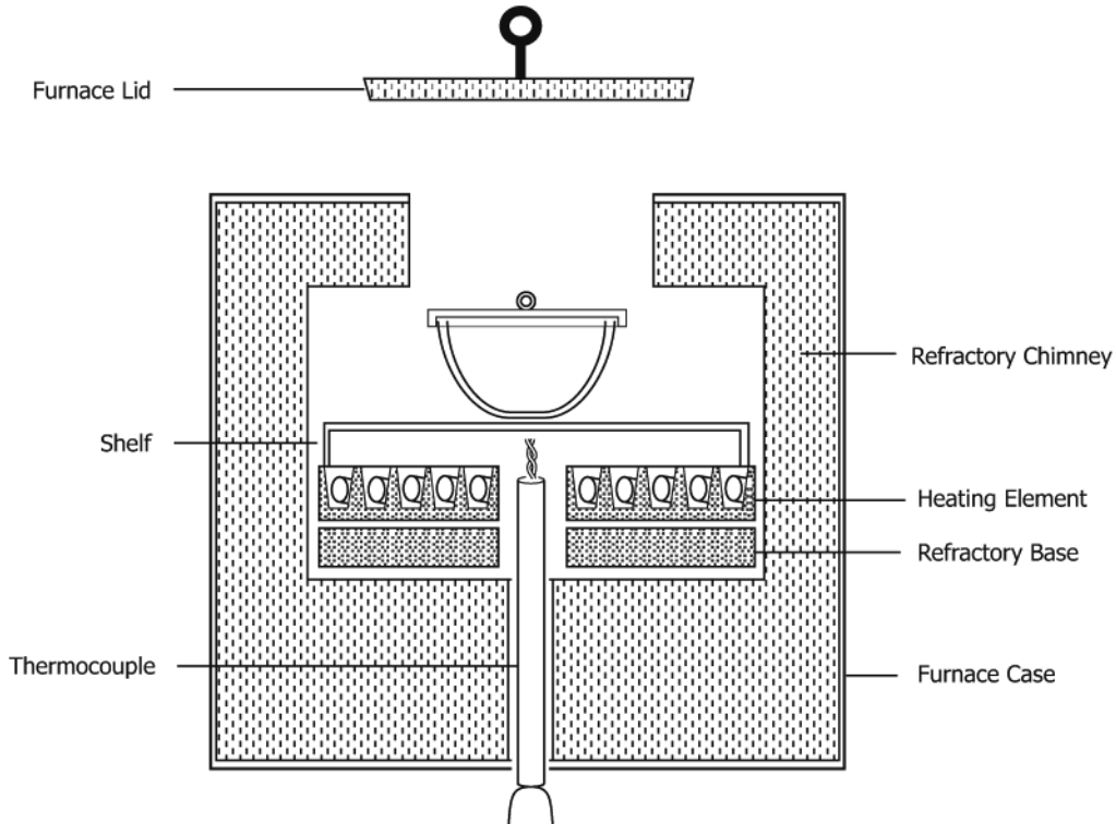
FIG. 2 Example Furnace Base and Chimney
